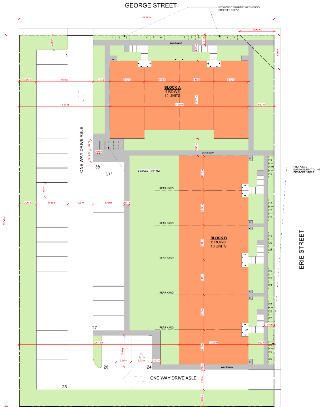
1 SITE PLAN A100 1:150
